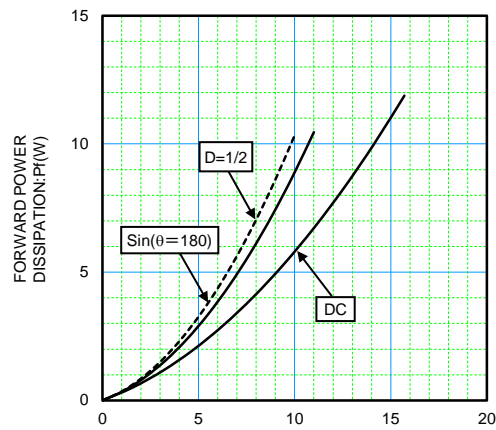
Io-Pf CHARACTERISTICS
