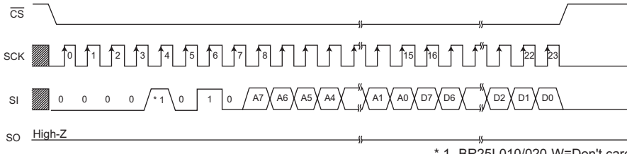
Fig.39 Write command (BR25L010/020/040-W) * 1 BR25L010/020-W=Don't care BR25L040-W=A8
