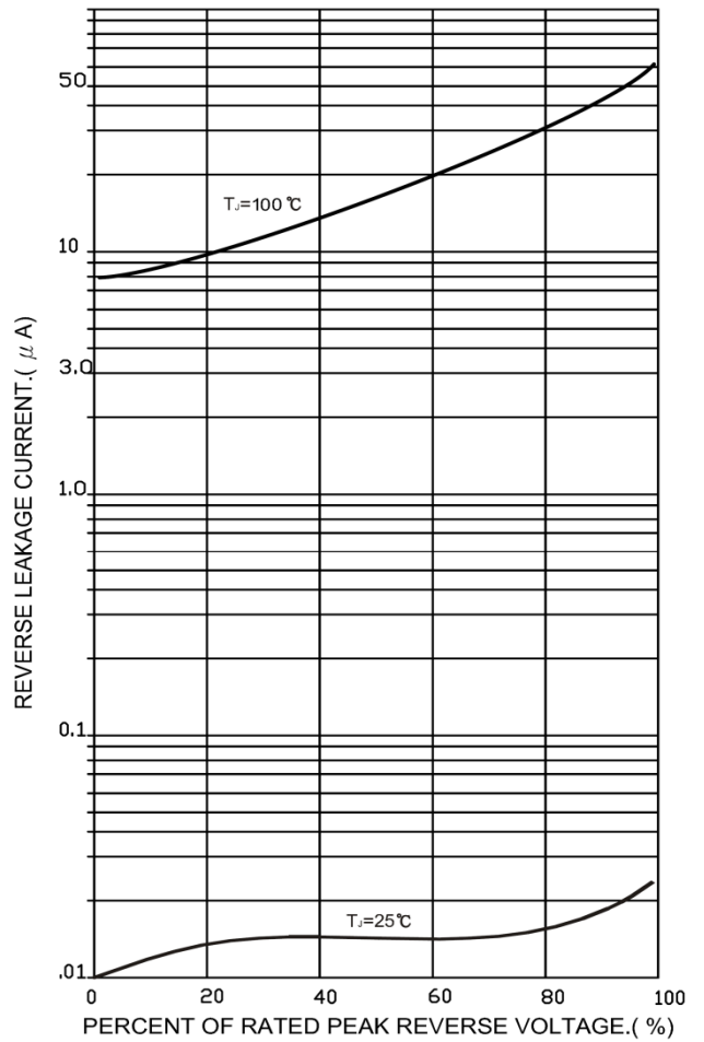
FIG.4-TYPICAL REVERSE CHARACTERISTICS
