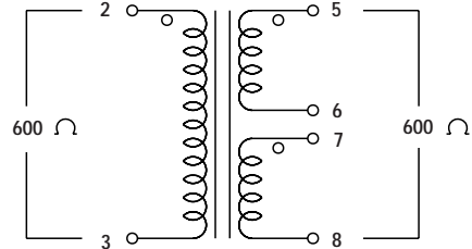
Schematic 7 (TTPC-Series)
