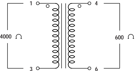
Schematic 8 (TTPC-Series)
