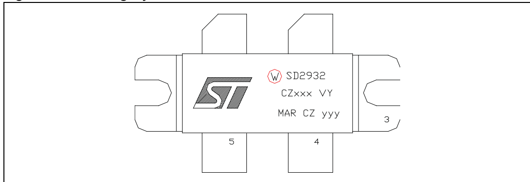
Figure 32. Marking layout
