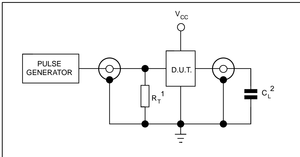
Figure 3: Test circuit
