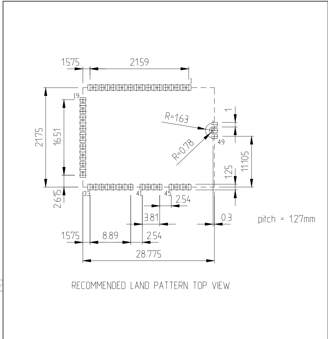
Figure 10. Mechanical dimensions
