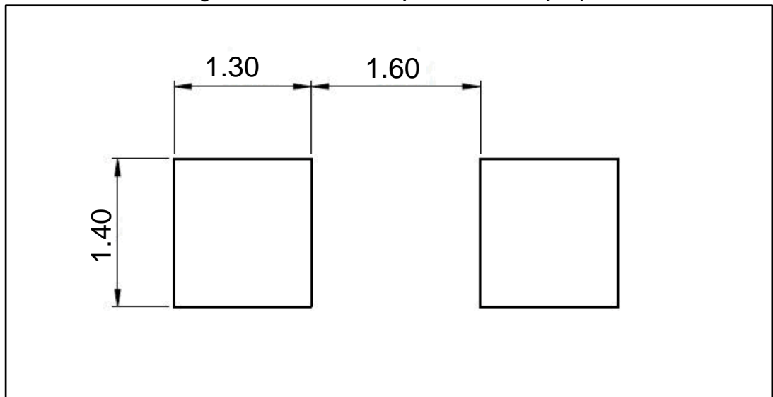
Figure 24: SOD123Flat footprint dimensions (mm)
