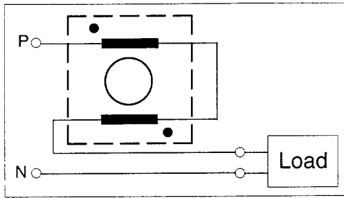
Functional schematic
