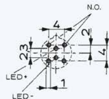
Drilling diagram
