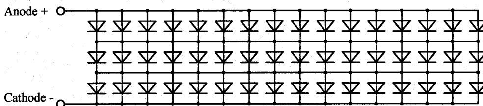
Equivalent circuit
