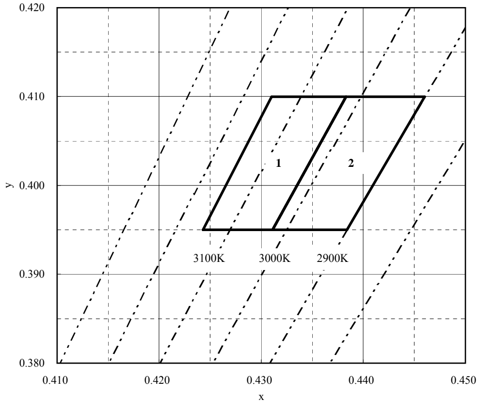
Chromaticity Diagram
