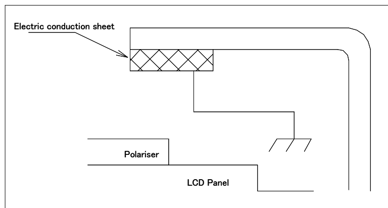
Figure 15-1 Design example
