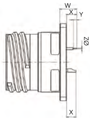
Type 21: Square flange receptacle
