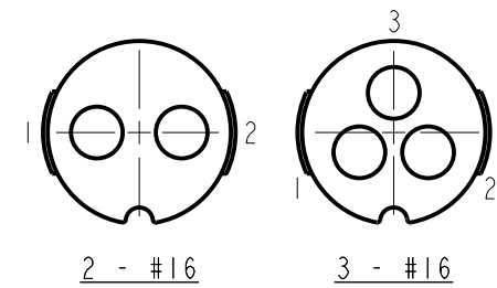
CONTACT ARRANGEMENTS
