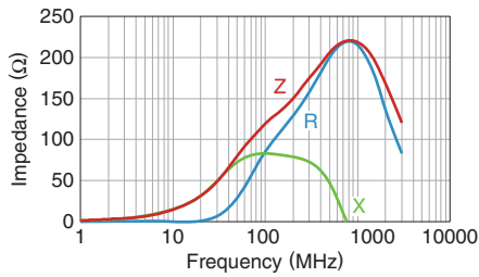
MMZ1005Y121C
