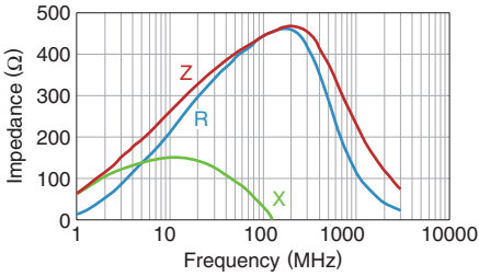
MPZ1608S600ATAH0
