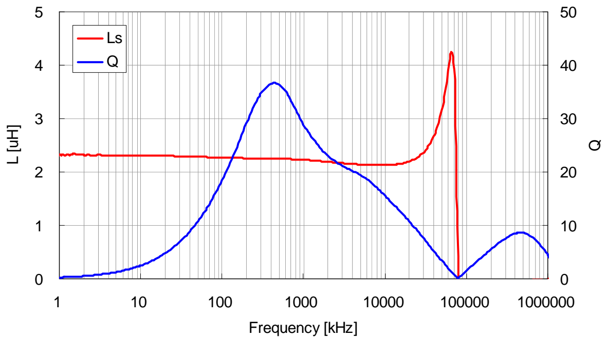
VLF4014ST-2R2M1R9
