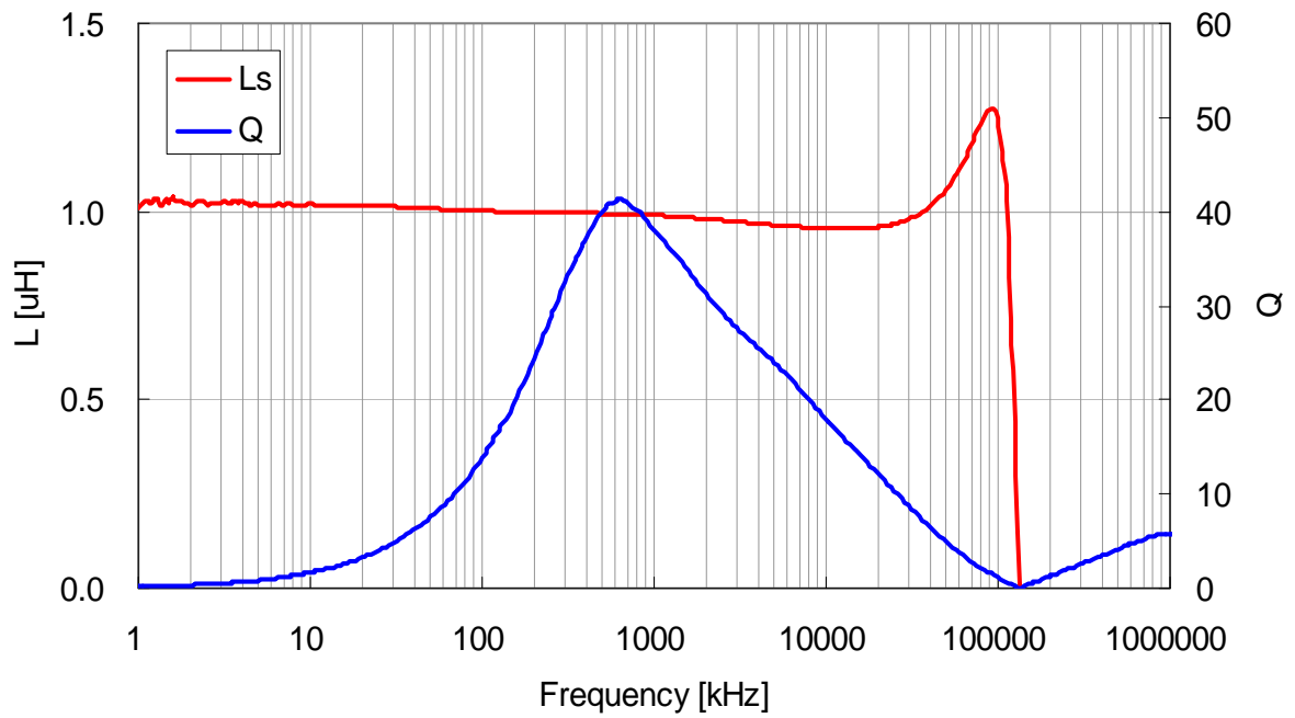
VLF4014ST-1R0N2R3
