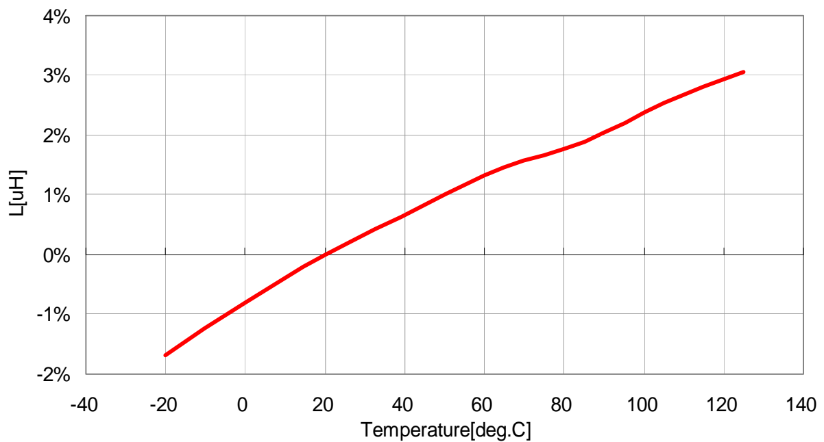
VLF4014ST-2R2M1R9
