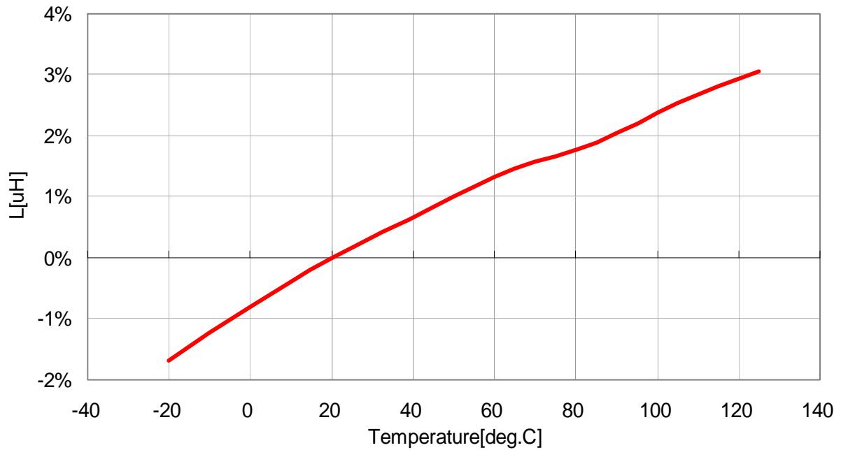
VLF4014ST-1R0N2R3
