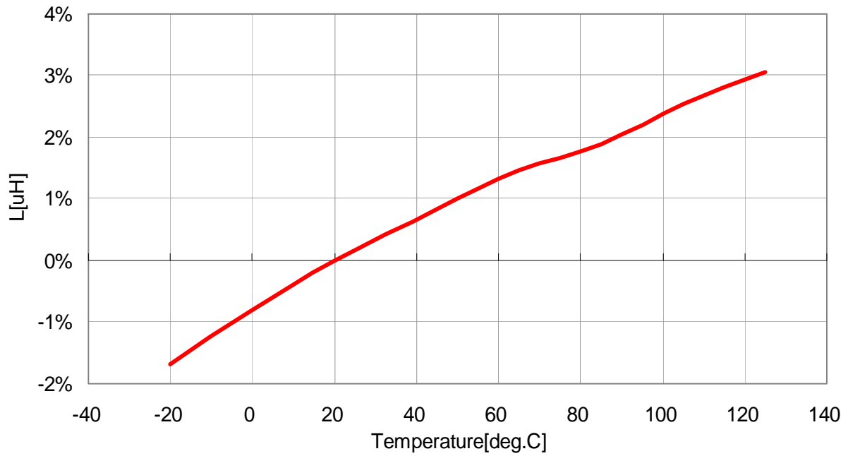
VLF4014ST-6R8M2R2
