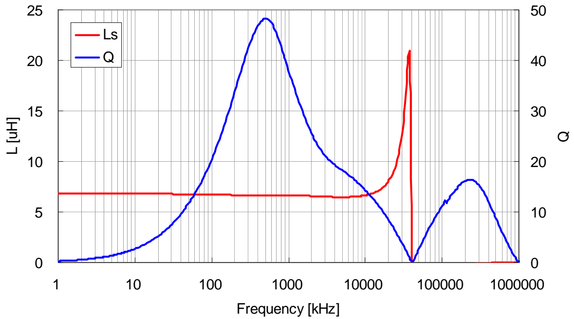
VLF4014ST-6R8M2R2
