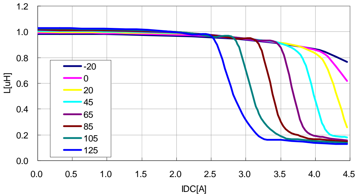
VLF4014ST-2R2M1R9
