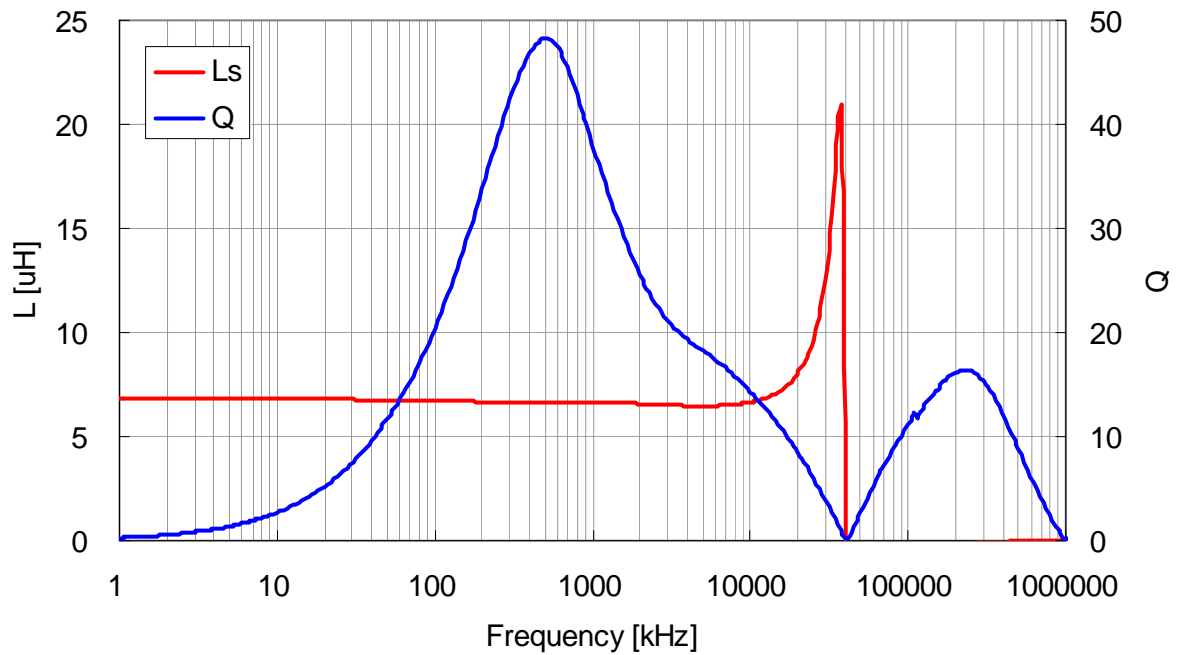
VLF4014ST-6R8M2R2
