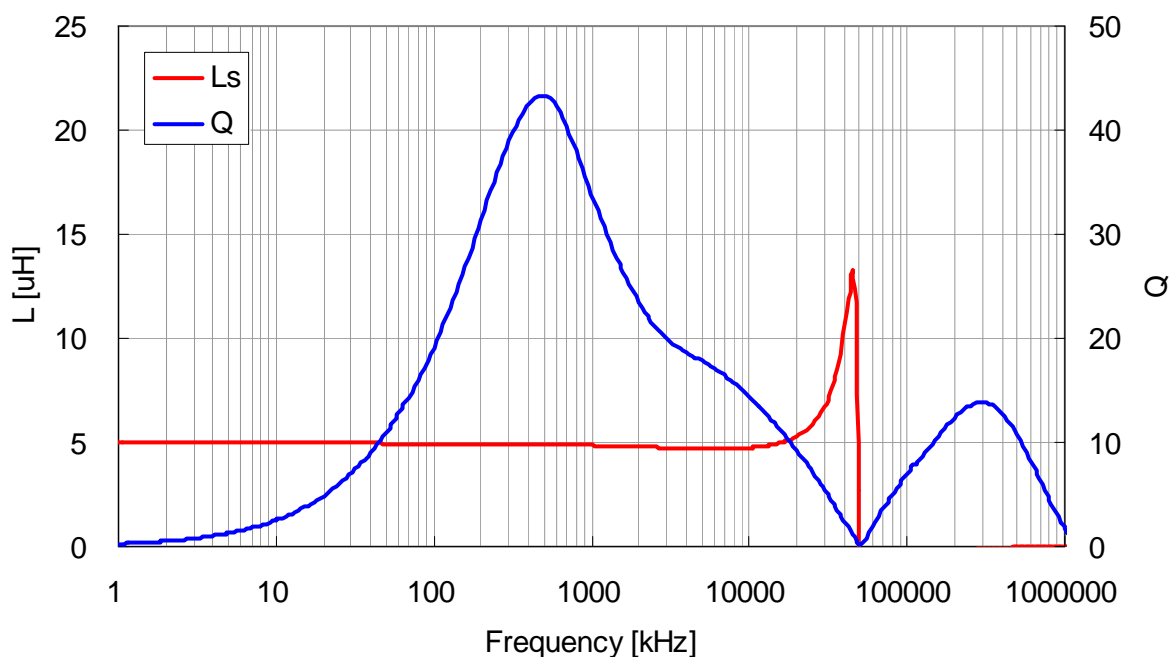
VLF4014ST-4R7M1R4
