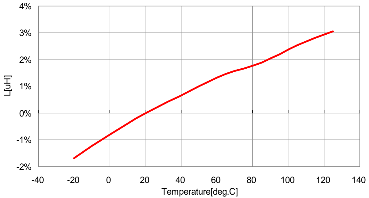
VLF4014ST-1R0N2R3
