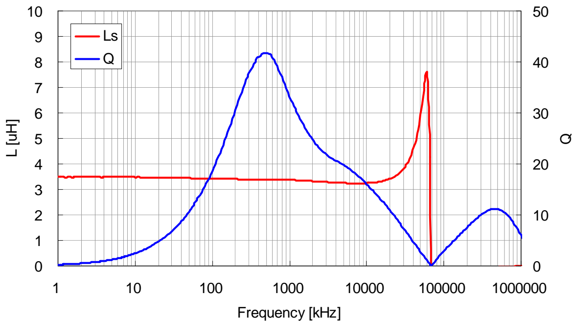
VLF4014ST-3R3M1R6
