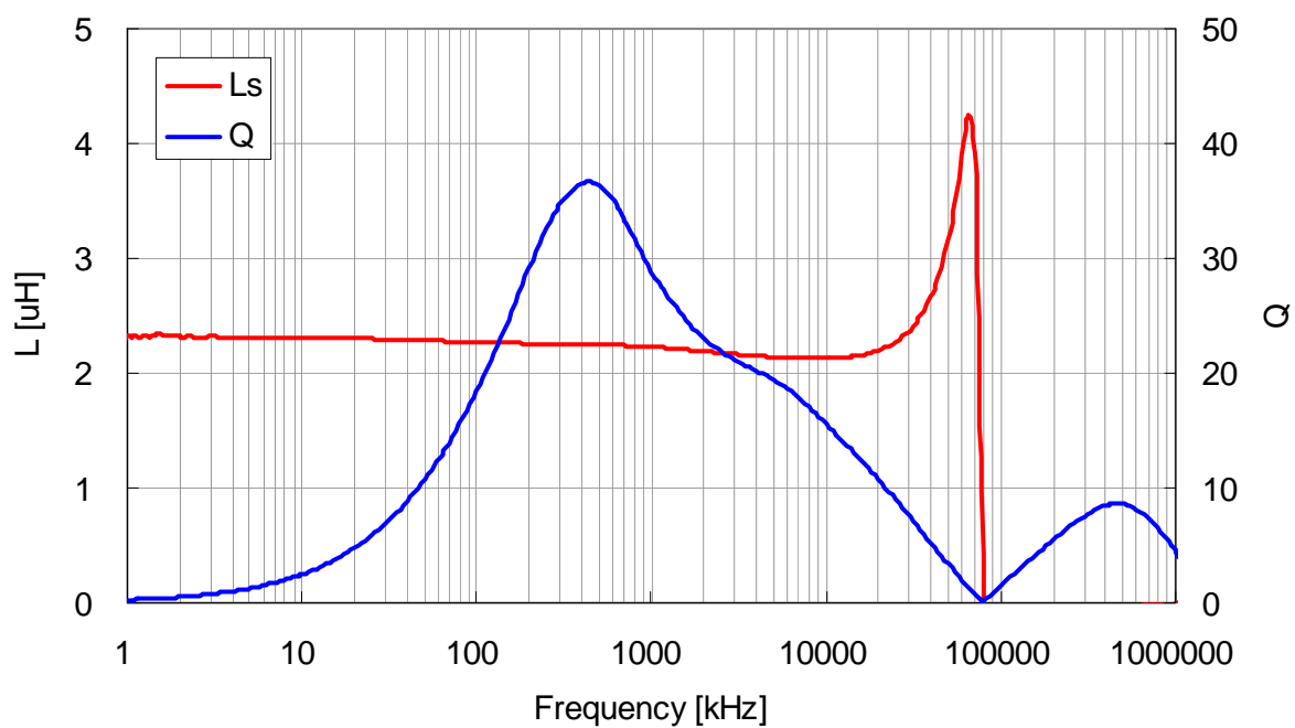
VLF4014ST-2R2M1R9
