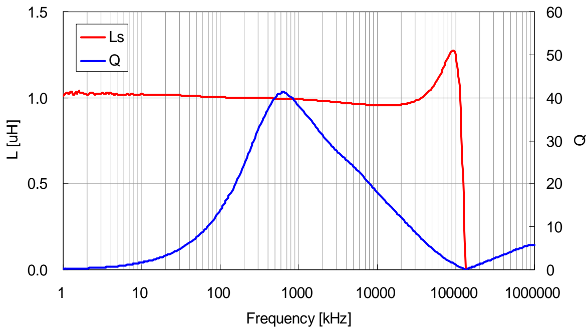
VLF4014ST-1R0N2R3
