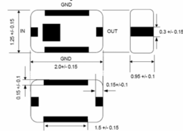
[MECHANICAL DIMENSIONS]
