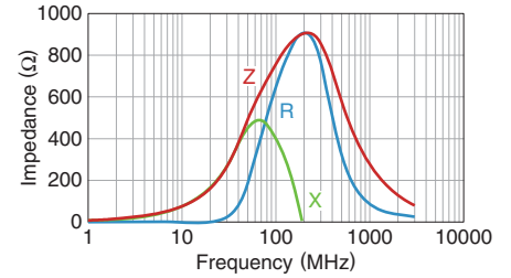
MMZ1608Y751B
