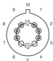
TERMINAL NUMBERING
