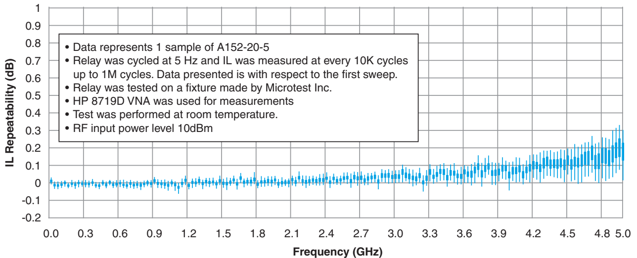
A152 Insertion Loss Repeatability (Attenuated Path)
