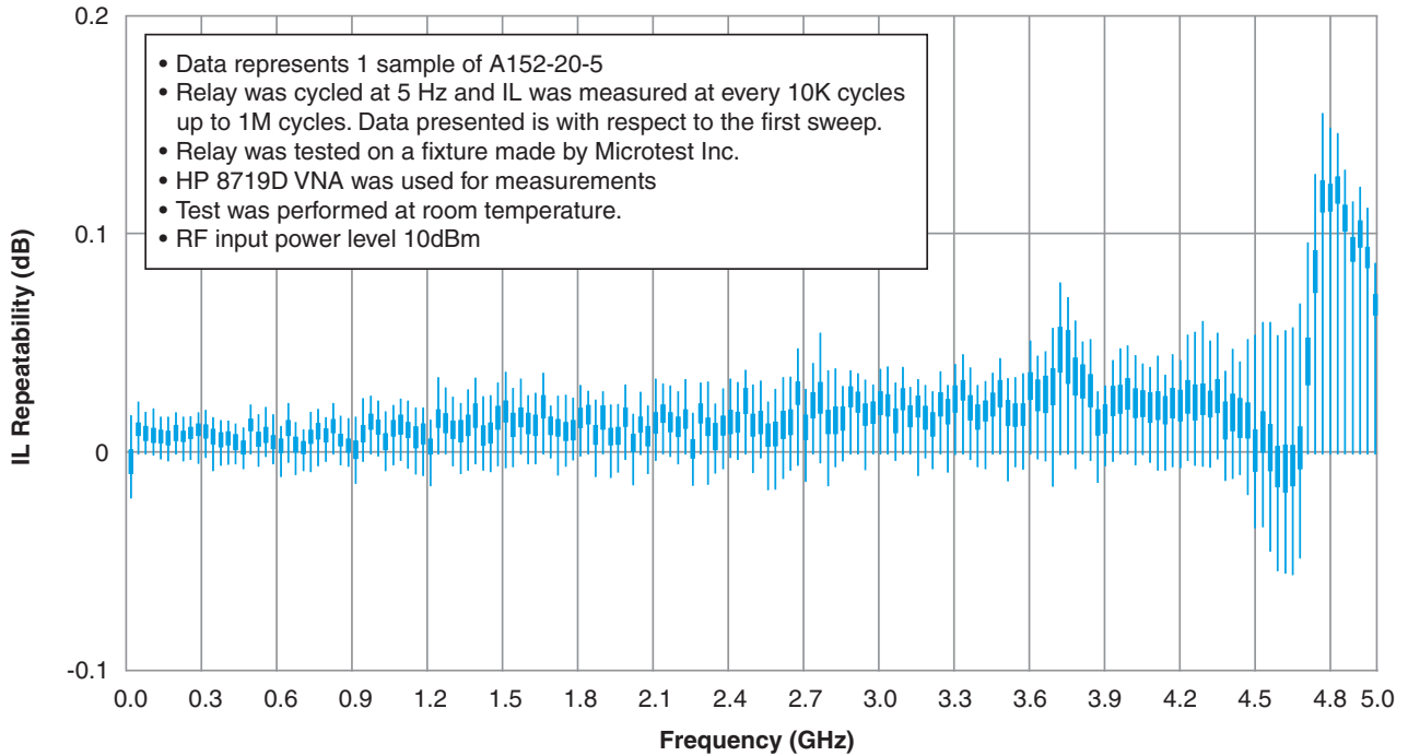
A152 Insertion Loss Repeatability (Through Path)
