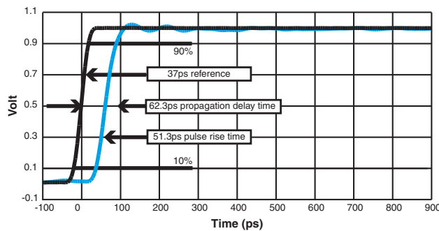
SGRF312/SGRF332 Time Response (RF Note 6)
