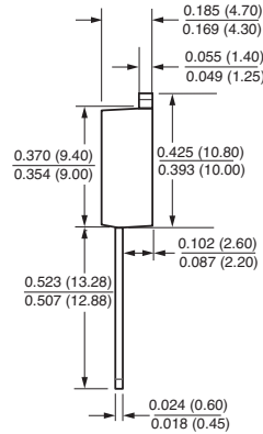
TO-262AA
