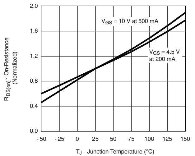
V_{GS} = 10 V at 500 mA V_{GS} = 4.5 V at 200 mA On-Resistance vs. Junction Temperature
