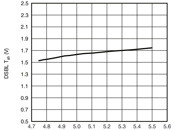
DSBL Rising Threshold vs. V CIN
