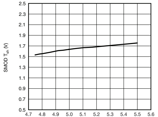
SMOD Rising Threshold vs. V CIN
