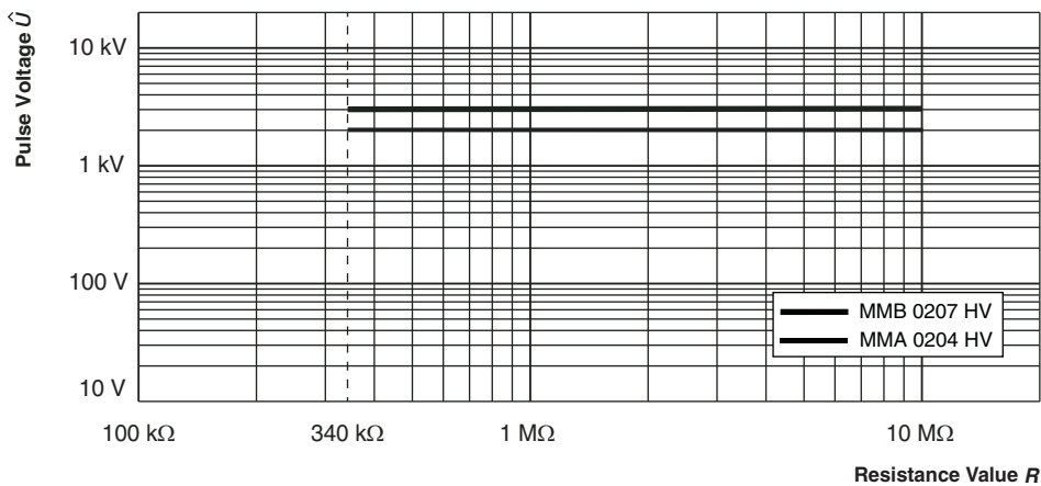
Pulse load rating in accordance with IEC 60 115-1, 4.27; 1.2 μs/50 μs; 5 pulses at 12 s intervals; for permissible resistance change (0.5 \% \times R + 0.05 \Omega)
