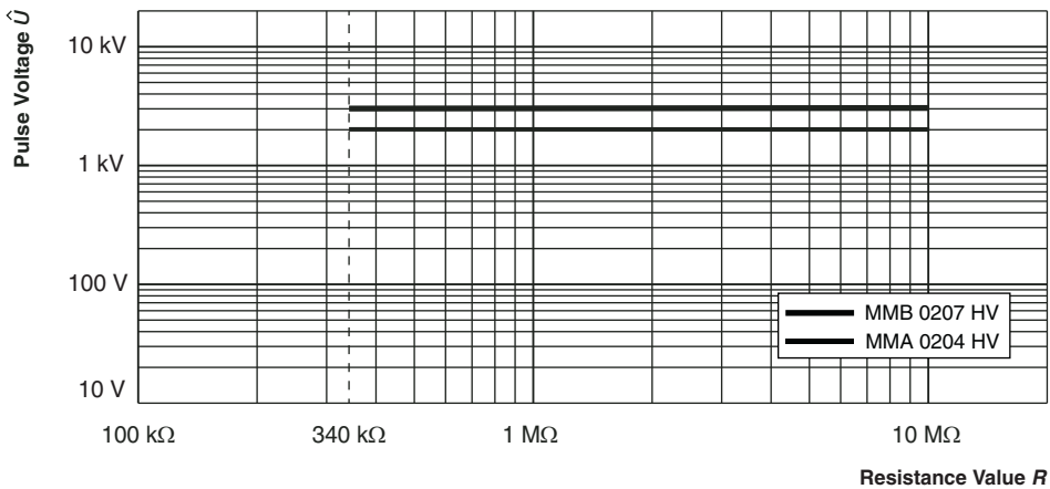
Pulse load rating in accordance with IEC 60115-1, 4.27; 10 μs/700 μs; 10 pulses at 1 minute intervals; for permissible resistance change (0.5 \% \times R + 0.05 \Omega)
