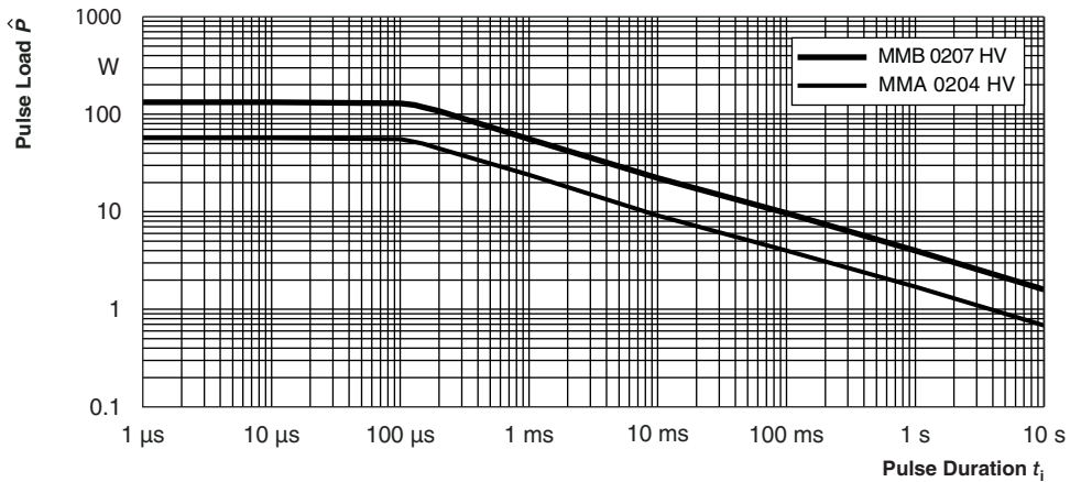
Maximum pulse load, continuous pulse; applicable if \hat{P} \leq P(\vartheta_{amb}) and \hat{U} \leq \hat{U}_{max} ; for permissible resistance change \pm (0.5 \% R + 0.01 \Omega)
