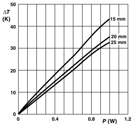
Ø 0.58 mm Cu-leads Minimum distance from resistor body to PCB = 1 mm PR01 Temperature rise ( \Delta T ) at the lead end (soldering point) as a function of dissipated power at various lead lengths after mounting.
