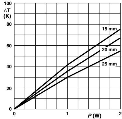
Ø 0.78 mm Cu-leads Minimum distance from resistor body to PCB = 1 mm PR02 Temperature rise ( \Delta T ) at the lead end (soldering point) as a function of dissipated power at various lead lengths after mounting.
