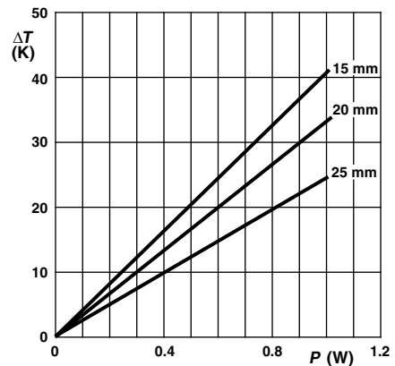
Ø 0.58 mm FeCu-leads Minimum distance from resistor body to PCB = 1 mm PR01 Temperature rise ( \Delta T ) at the lead end (soldering point) as a function of dissipated power at various lead lengths after mounting.
