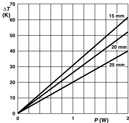
Ø 0.58 mm FeCu-leads Minimum distance from resistor body to PCB = 1 mm PR02 Temperature rise ( \Delta T ) at the lead end (soldering point) as a function of dissipated power at various lead lengths after mounting.
