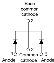
VS-40CTQ045-1PbF
