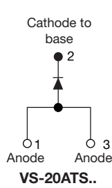
TO-220AB
