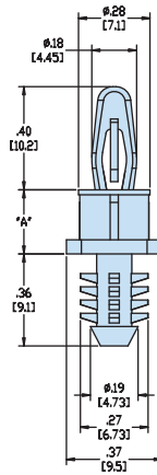
BAYONET SNAP LOCK 10,2 / BLIND FIR TREE
