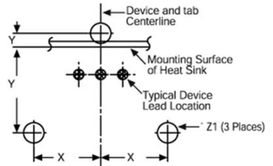
Mounting Details:
