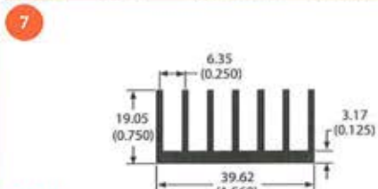
class A 61080 0.5 lb/ft 5.79 °C/W/3in Per.=12.07
