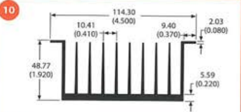
77915 2.6 lb/ft 1.67 °C/W/3in Per.=41.99
