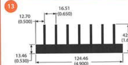
13 80965 4.2 lb/ft 2.61 °C/W/3in Per.=26.82
