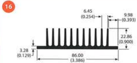
81850 1.3 lb/ft 3.08 °C/W/3in Per.=22.71
