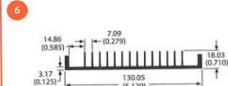
78950 2.7 lb/ft 1.76 °C/W/3in Per.=39.78
