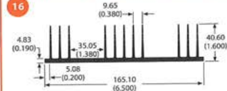
61715 2.8 lb/ft 1.62 °C/W/3in Per.=43.19
