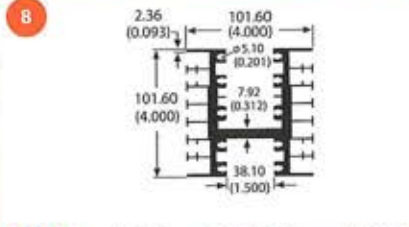
61270 5.1 lb/ft 1.13 °C/W/3in Per.=61.84
