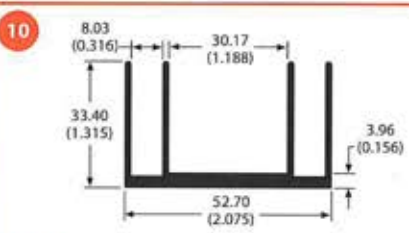
62355 0.7 lb/ft 5.10 °C/W/3in Per.=13.71
