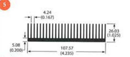
class A 74765 2.4 lb/ft 1.38 °C/W/3in Per.=50.53
