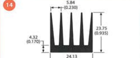
64675 0.5 lb/ft 7.40 °C/W/3in Per.=9.45
