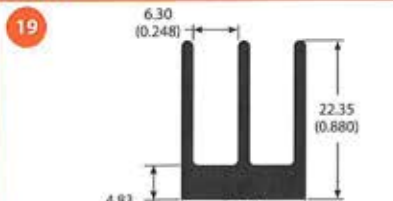
64640 0.1 lb/ft 18.07 °C/W/3in Per.=3.87
