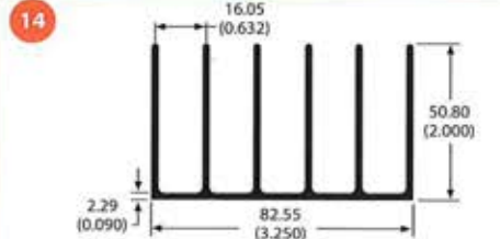
62875 1.6 lb/ft 2.41 °C/W/3in Per.=29.03
