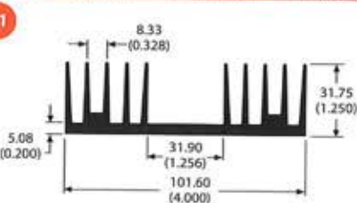
82350 2.1 lb/ft 2.52 °C/W/3in Per.=27.78
