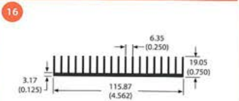
class A 60585 1.5 lb/ft 2.15 °C/W/3in Per.=32.46
