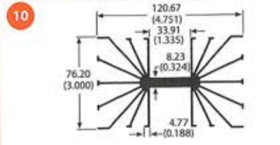
60650 2.9 lb/ft 1.14 °C/W/3in Per.=61.23
