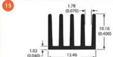
class A 62000 0.1 lb/ft 15.30 °C/W/3in Per.=4.57
