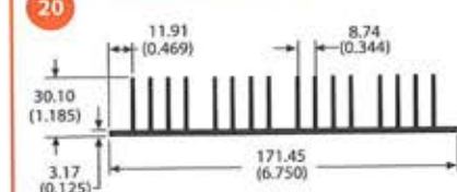
60995 2.6 lb/ft 1.50 °C/W/3in Per.=46.59
