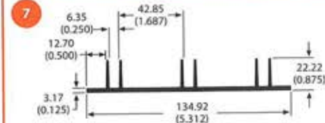
68830 1.4 lb/ft 2.52 °C/W/3in Per.=27.79
