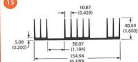
61690 2.6 lb/ft 1.64 °C/W/3in Per.=42.51
