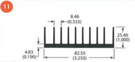
class A 60760 1.3 lb/ft 3.11 °C/W/3in Per.=22.50
