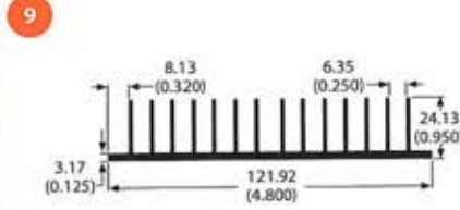
79025 1.5 lb/ft 2.15 °C/W/3in Per.=32.47
