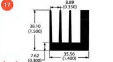
class A 61605 1.2 lb/ft 5.47 °C/W/3in Per.=12.78
