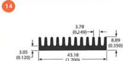
79920 0.5 lb/ft 8.38 °C/W/3in Per.=8.34
