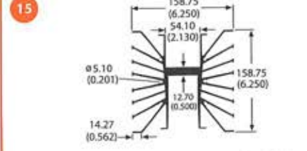
60265 7.7 lb/ft 0.67 °C/W/3in Per.=104.01
