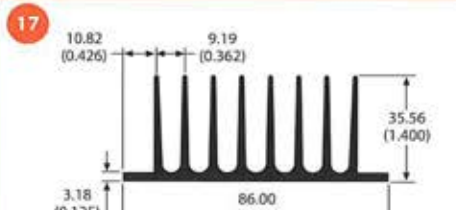
81855 1.6 lb/ft 2.68 °C/W/3in Per.=26.09
