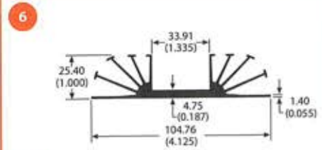
class A 60080 1.2 lb/ft 2.91 °C/W/3in Per.=24.04
