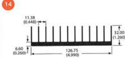
class A 61745 2.4 lb/ft 2.06 °C/W/3in Per.=33.89
