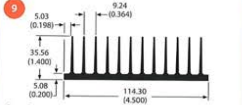
class A 61075 2.3 lb/ft 1.90 °C/W/3in Per.=36.83
