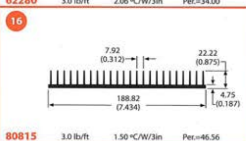
80815 3.0 lb/ft 1.50 °C/W/3in Per.=46.56
