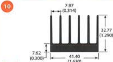
class A 61215 1.0 lb/ft 4.54 °C/W/3in Per.=15.40
