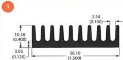
79940 0.4 lb/ft 8.63 °C/W/3in Per.=8.11
