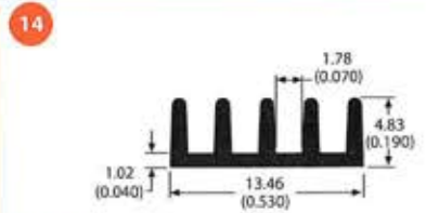
class A 61945 0.1 lb/ft 27.86 °C/W/3in Per.=2.51
