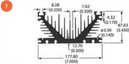
64730 10.9 lb/ft 0.75 °C/W/3in Per.=93.19
