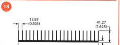
class A 62325 10.8 lb/ft 0.82 °C/W/3in Per.=85.27
