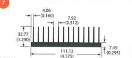
class A 60560 2.6 lb/ft 1.91 °C/W/3in Per.=36.52
