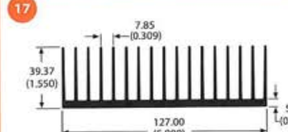
class A 67895 1.4 lb/ft 2.38 °C/W/3in Per.=29.33
