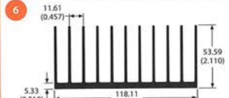
70970 3.2 lb/ft 1.38 °C/W/3in Per.=50.60
