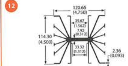
60060 4.0 lb/ft 0.98 °C/W/3in Per.=71.03
