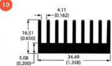
80595 0.6 lb/ft 6.38 °C/W/3in Per.=10.96
