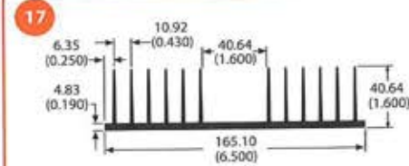
61715 2.8 lb/ft 1.62 °C/W/3in Per.=43.19
