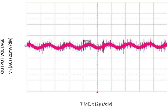
Fig 12: 3.3V Ripple
