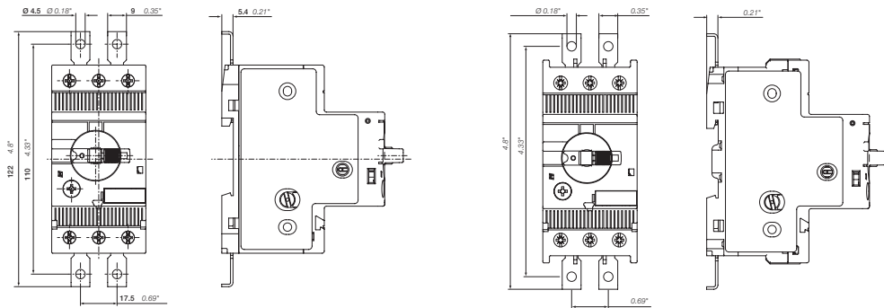
MS132-T ≤ 10 A with screw fixing kit FS116 (accessory)
