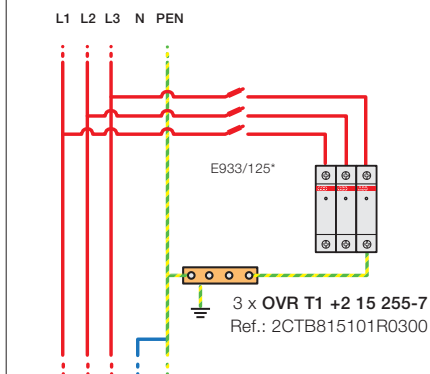
Configuration 3 I_p \leq 7 \text{ kA}
