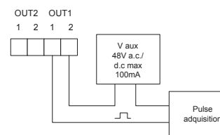
Digital output used as pulses
