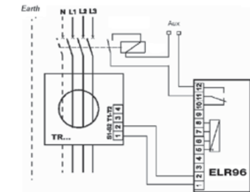
ELR96 - shunt trip wiring
