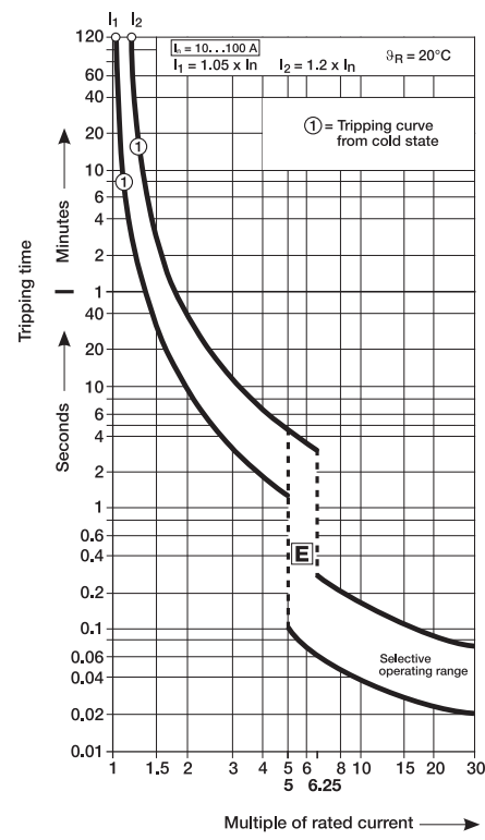
Characteristic E selective S 750 DR - 16 ... 25 A
