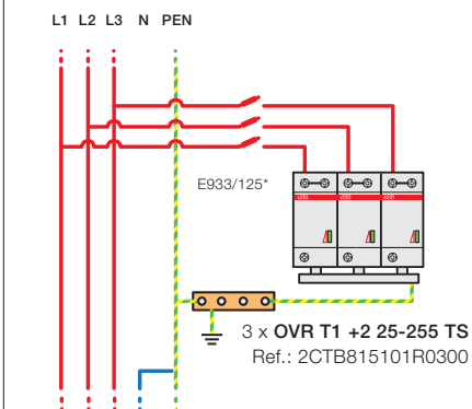
Configuration 2 7 \text{ kA} \leq I_p \leq 15 \text{ kA}
