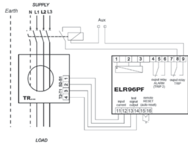
ELR96PF - shunt trip wiring
