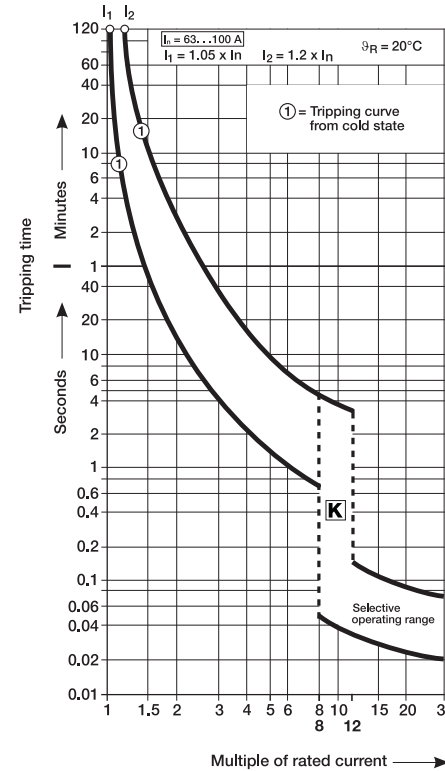
Characteristic K selective S 700 - 63 ... 100 A
