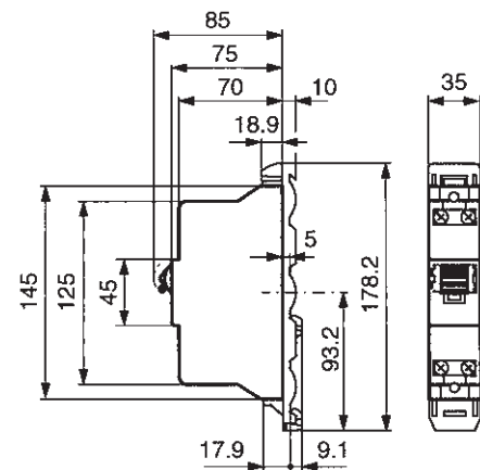
S 701 with DIN rail adapter
