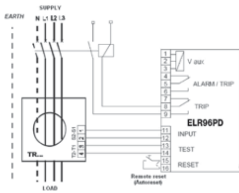
ELR96PD - shunt trip wiring
