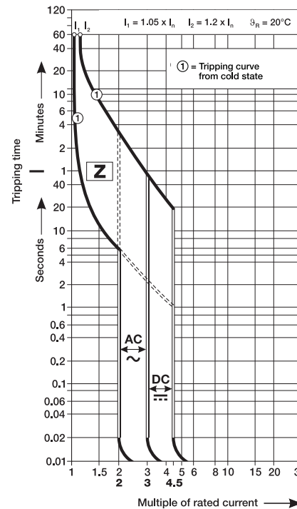
Z characteristic
