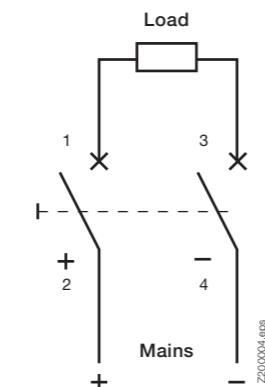
Connection diagram, two-pole (max. 250 V=) S402M-UCC
