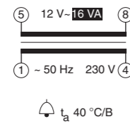
TS16/4-8-12
