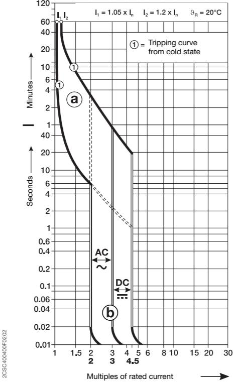
Characteristic Z IEC-EN60947-2
