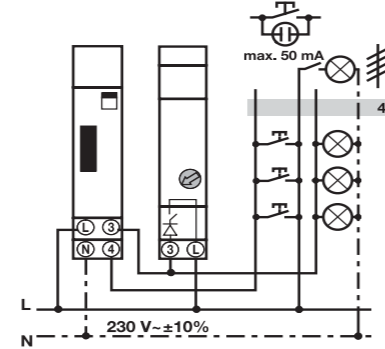
E 232 HLM 4 conductor
