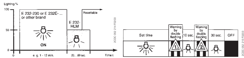
timing of a staircase lighting time-delay switch with semi-light module E 232-HLM
