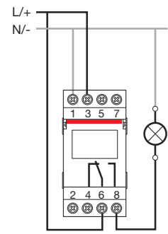
TWA-1
