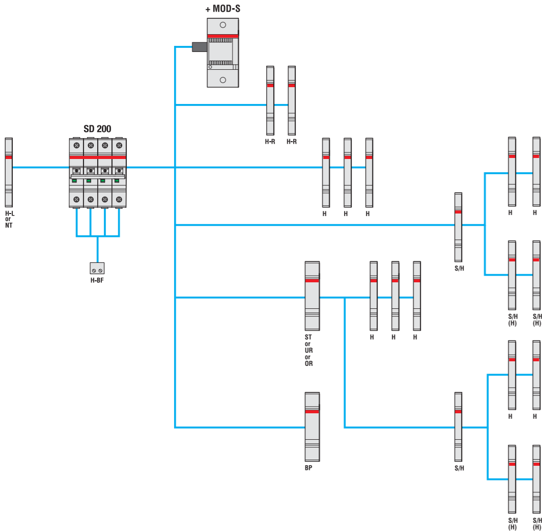
Combination of auxiliary elements with SD 200
