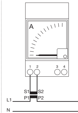
Indirect insertion using C.T.
