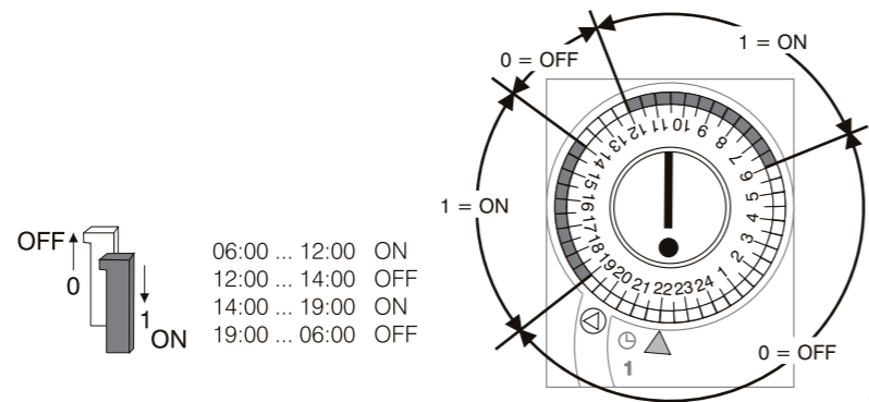
Switching dial
