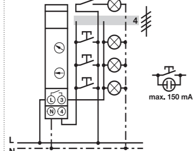
E 232E-230 Multi 10 4 conductor
