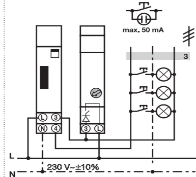
E 232 HLM 3 conductor
