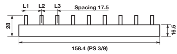
PS 3/9
