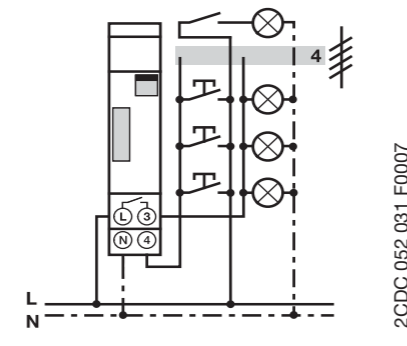
E 232-230 4 conductor
