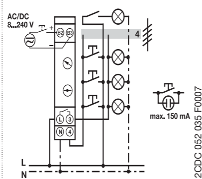
E 232E-8/230 Multi 10 4 conductor
