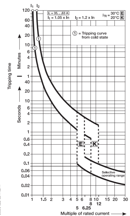
Characteristic K selective S 750 DR - 35 ... 63 A
