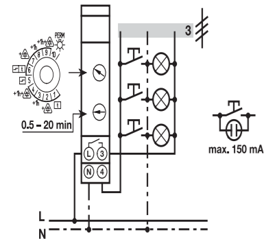
E 232E-230 Multi 10 3 conductor
