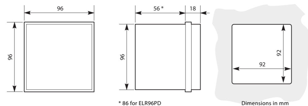
ELR96
