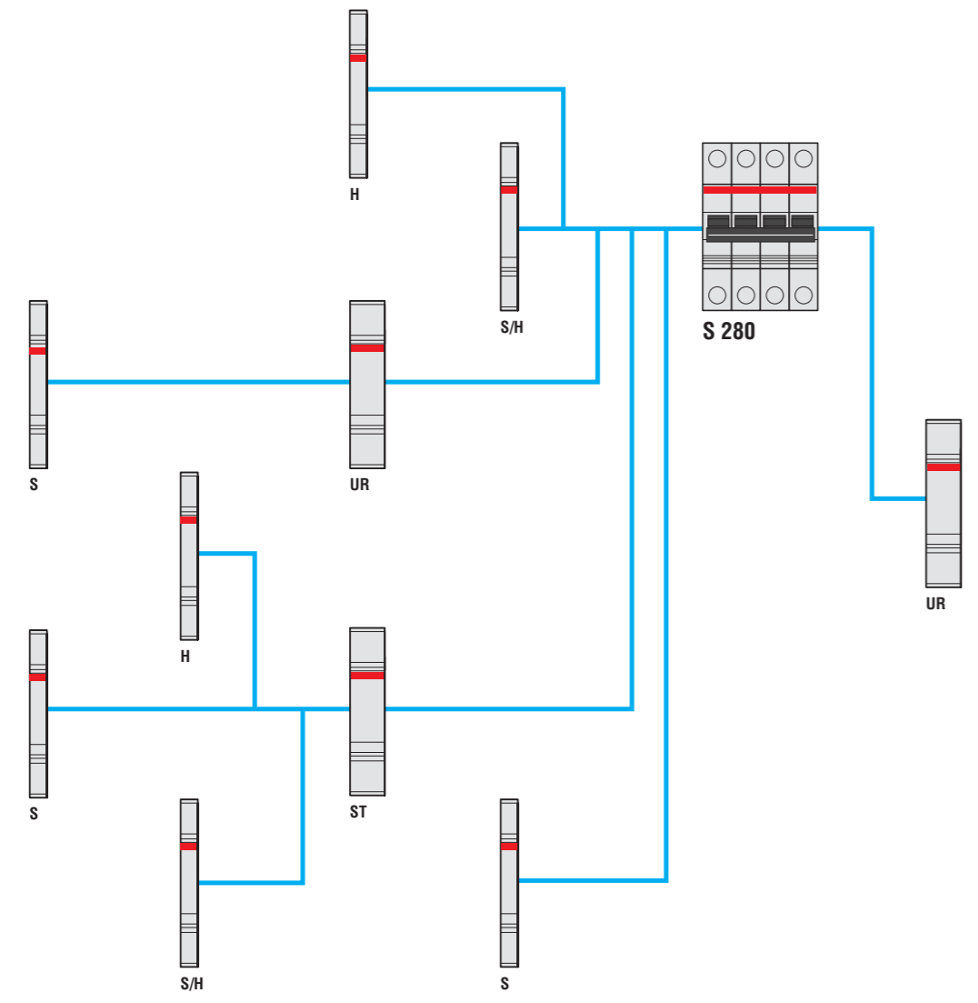
Combination between auxiliary elements and S 280
