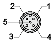
Adam M12-5 male connector. (Note that some models have 8 pins instead.)
