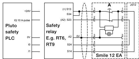
Dual channel - Safety category 4.
