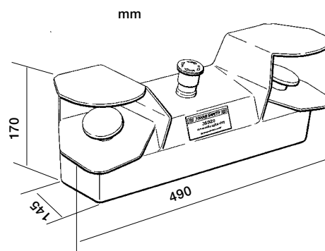
JSTD20A – Two-hand device, without emergency stop
