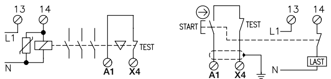
Controlled monitoring of external jockab safety's expansion relays.
