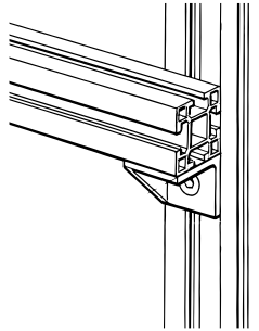
Angle fitting
