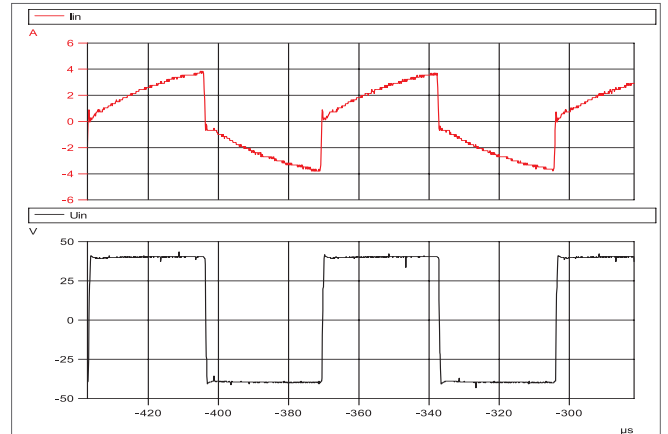
04 Typical waveform of input voltage and supply current when using square-wave AC supply
