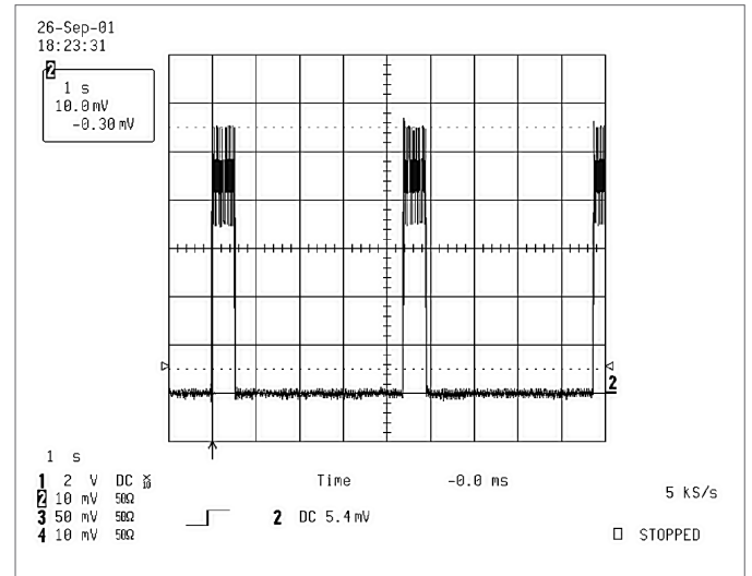
18 Power up during shorted gate unit load
