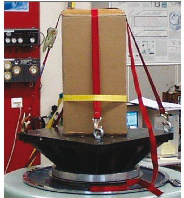
22 Vibration test with IGCTs wrapped in transport box
