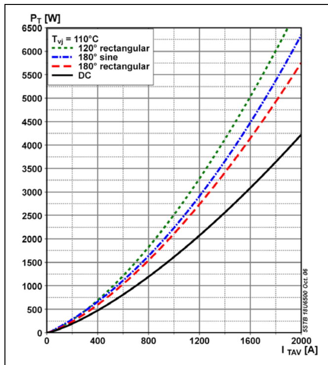
Fig. 4 On-state power dissipation vs. mean on-state current. Switching losses excluded.
