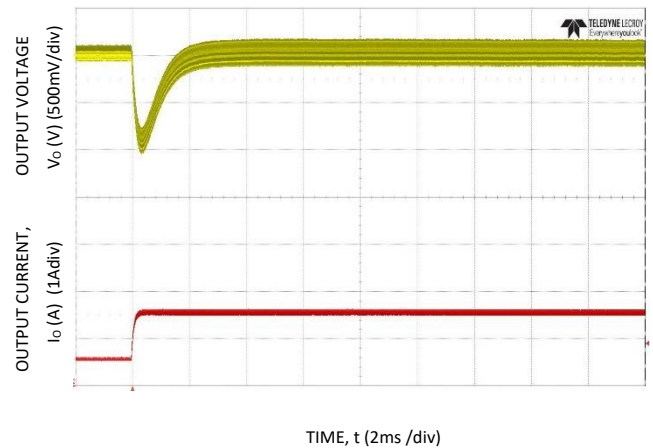
Figure 10. Transient Response to Dynamic Load Change from 0.6 to 1.6A at 12Vin, C_{out}=10x4.7\mu\text{F} , C_{Tune}=560\text{pF} , R_{Tune}=40.2\text{k}
