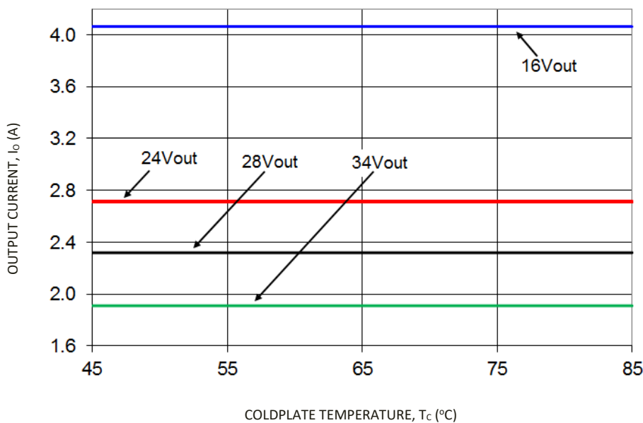
Figure 34. Output Current versus Coldwall Temperature; V_{IN} = 12V .
