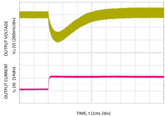
Figure 16. Transient Response to Dynamic Load Change from 50% to 100% at 12Vin, C out =9x10µF, CTune=3300pF, RTune=30.1kΩ
