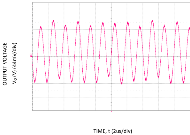
Figure 21. Typical output ripple and noise ( C_o=3x10uF+470uF , V_{IN} = 12V , I_o = I_{o,max} ).
