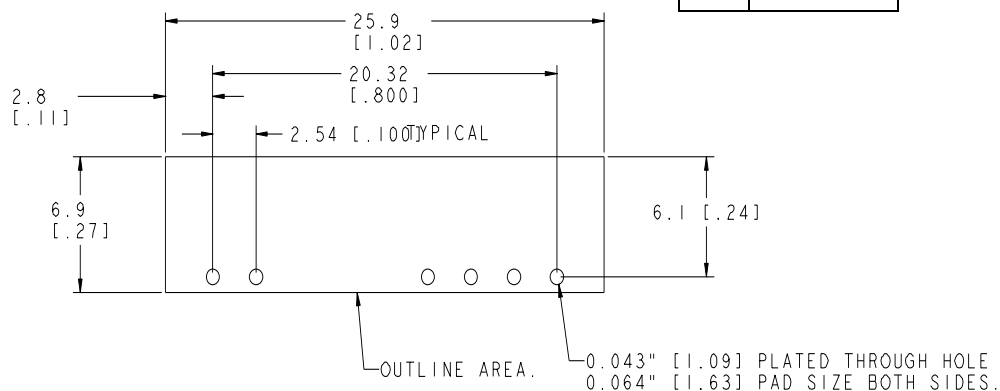
Through Hole Pad Layout – Back view
