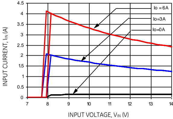
Figure 7. Input voltage vs. Input Current ( V_{out} = 5Vdc ).
