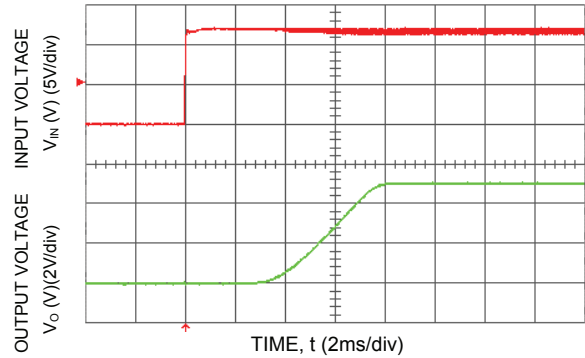
Figure 16. Typical Start-Up with application of V_{in} with low-ESR polymer capacitors at the output (7x150 \mu F) ( V_{in} = 12 Vdc, V_o = 5.0 Vdc, I_o = 10 A)
