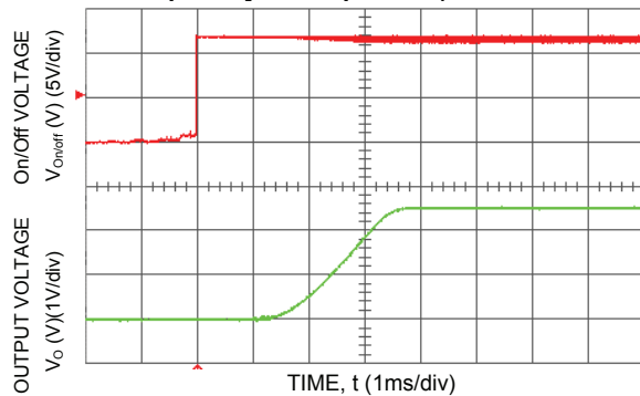
Figure 14. Typical Start-Up Using Remote On/Off ( V_{in} = 12 Vdc, V_o = 5.0 Vdc, I_o = 10 A).
