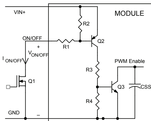
Figure 27. Circuit configuration for using positive logic On/Off.
