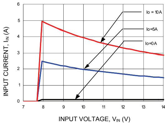
Figure 7. Input voltage vs. Input Current ( V_o = 2.5Vdc ).
