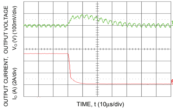
Figure 13. Transient Response to Dynamic Load Change from 100% of 50% full load ( V_o = 3.3 Vdc, C_{ext} = 2 \times 150 \mu F Polymer Capacitors).
