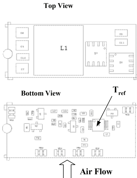
Figure 32. T_{ref} Temperature measurement location.
