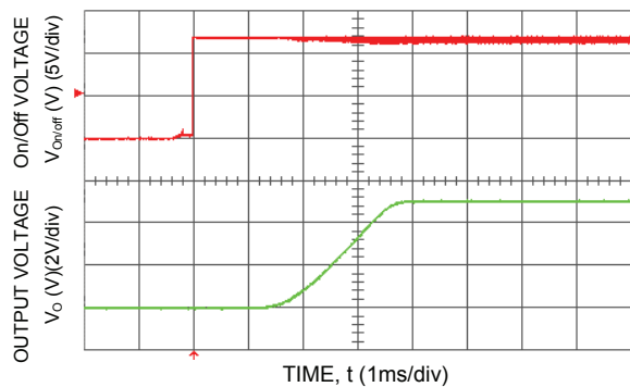
Figure 15. Typical Start-Up Using Remote On/Off with external capacitors ( V_{in} = 12.0 Vdc, V_o = 5.0 Vdc, I_o = 10 A, C_o = 1050 \mu F).
