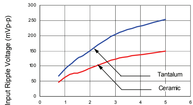
Figure 26. Input ripple voltage for various output with 4x47 µF tantalum capacitors and with 4x22 µF ceramic capacitors at the input (full load).
